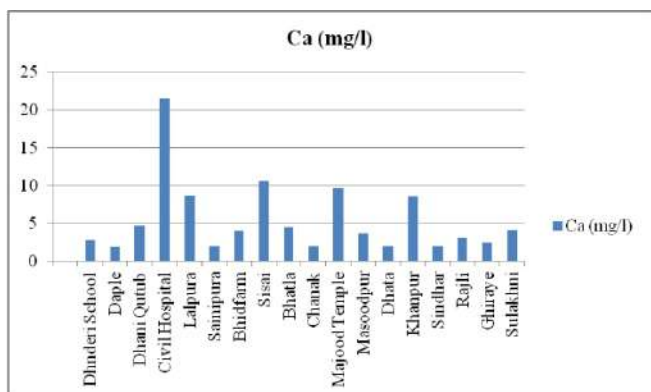
Fig.12: Scenario of calcium in groundwater samples in the study area.
