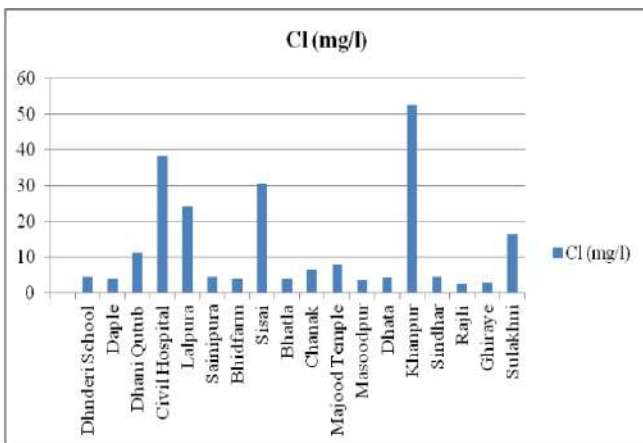
Fig.7: Scenarios of chloride in groundwater samples in the study area.
