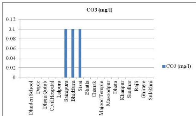
Fig.11: Scenario of carbonate in groundwater samples in the study area.
