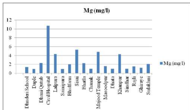
Fig.12: Scenario of magnesium in groundwater samples in the study area.
